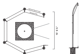
6 POLE DESIGN
