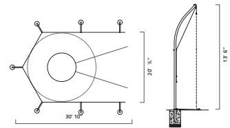
7 POLE DESIGN
