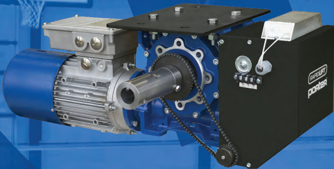
Curtain Winch
