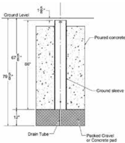
GROUND SLEEVE
